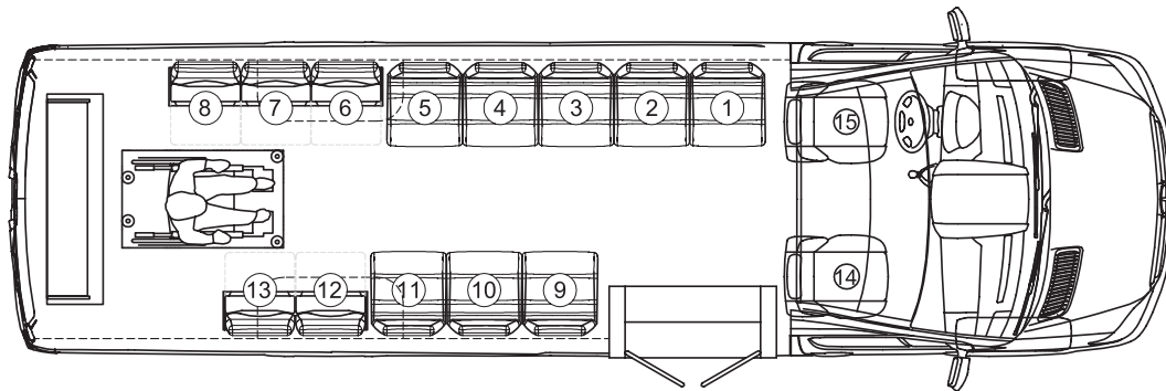
Sprinter MC15 Rear Lift Paratransit SPR-051
