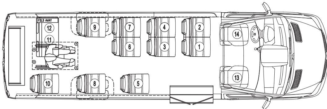
Sprinter MC14 Rear Lift Paratransit SPR-057
