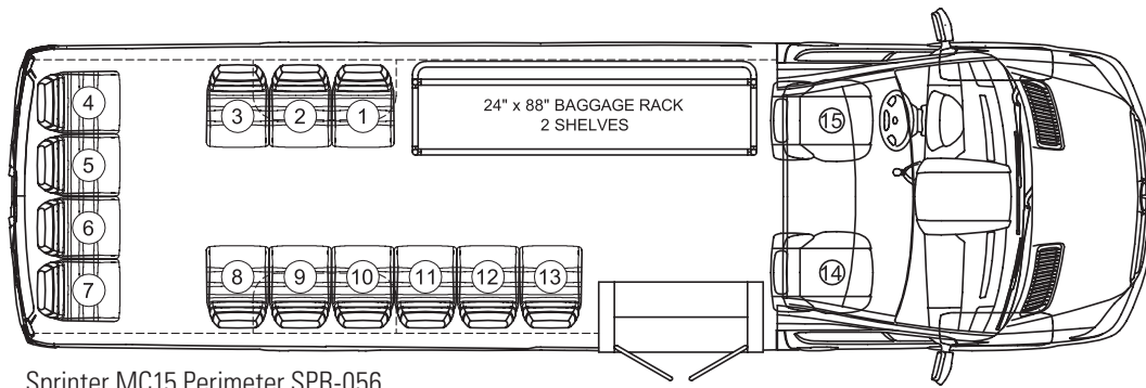
Sprinter MC15 Perimeter SPR-056
